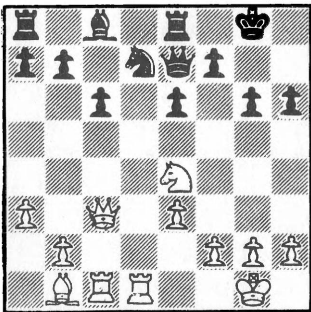
488 After 18...Bd5
